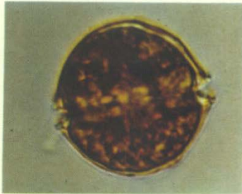
◀ Alexandrium tamarense
