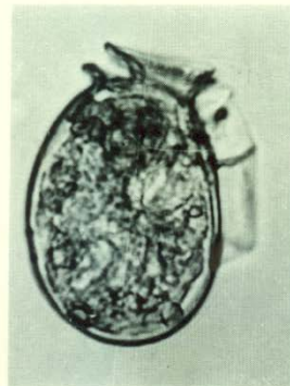
Dinophysis acuminata ▶
