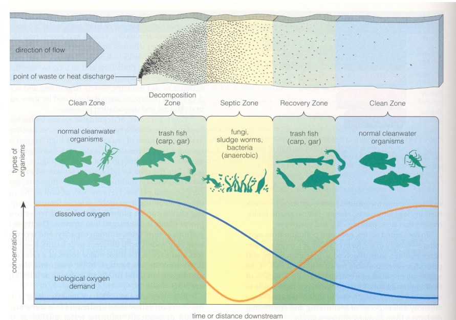
figure 11-22 Dilution and decay of degradable, oxygen-demanding wastes and heat, showing the oxygen sag curve (orange) and the curve of oxygen demand (blue). Depending on flow rates and the amount of pollutants, streams recover from oxygen-demanding wastes and heat if they are given enough time and are not overloaded.
